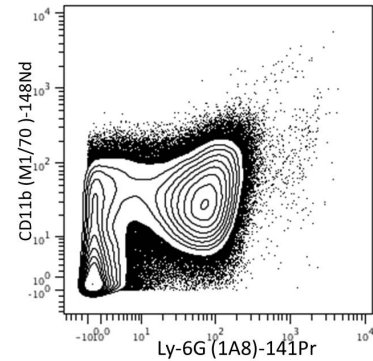
C57BL/6 mouse bone marrow cells stained with 148Nd-anti-CD11b (M1/70 ) and 141Pr-anti-Ly-6G (1A8).
