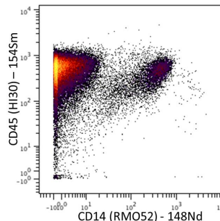
Human PBMCs stained with 154Sm-anti-CD45 (HI30) and 148Nd-anti-CD14 (RMO52).
